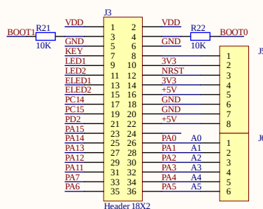
Header 18X2
