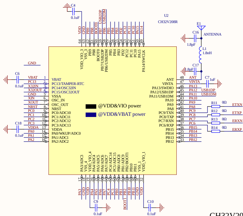
CH32V208R
